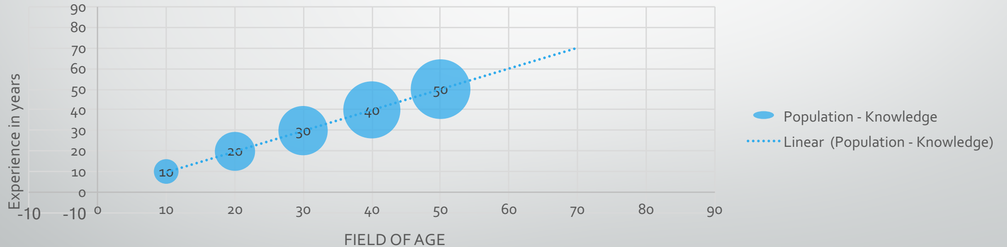
Population - Knowledge
